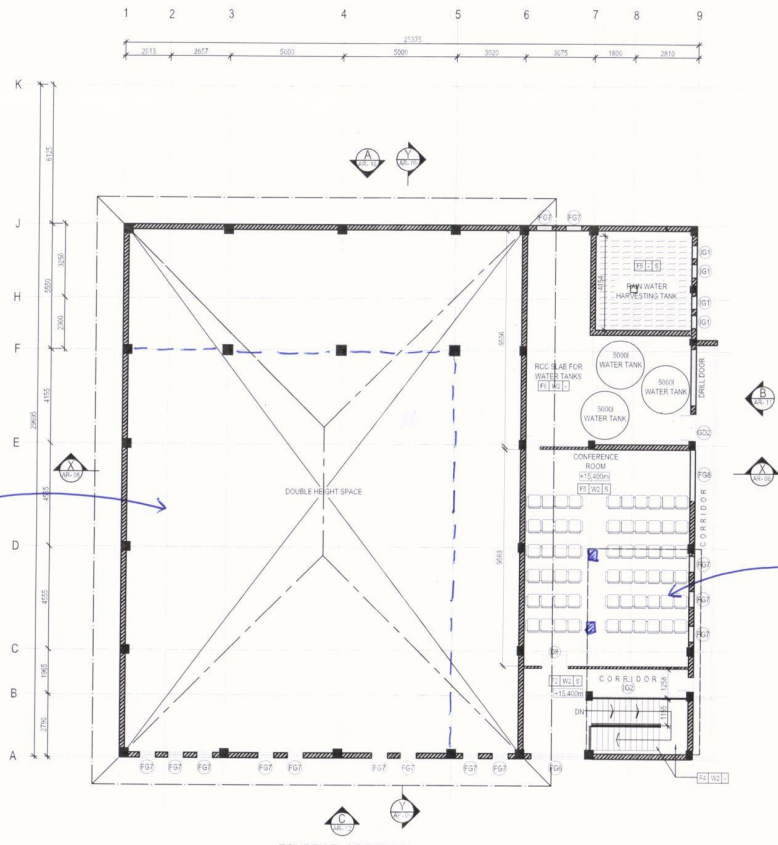
FOURTH FLOOR PLAN SCALE: 1/15 FLOOR AREA = 172.51 m 2
